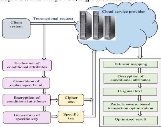
Figure 2. Architecture diagram of CSTAE-PSTO framework
